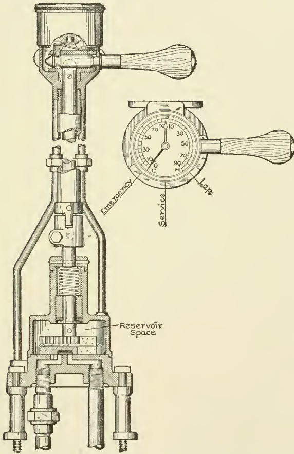
Fig. 96. Front View and Section of Another Form of Operating Valve
